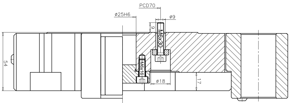
SECTION - FF
