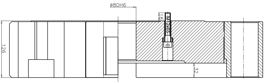
SECTION - FF
