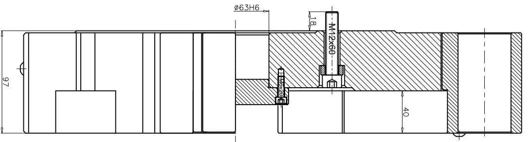
SECTION - FF
