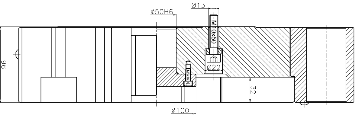
SECTION - FF
