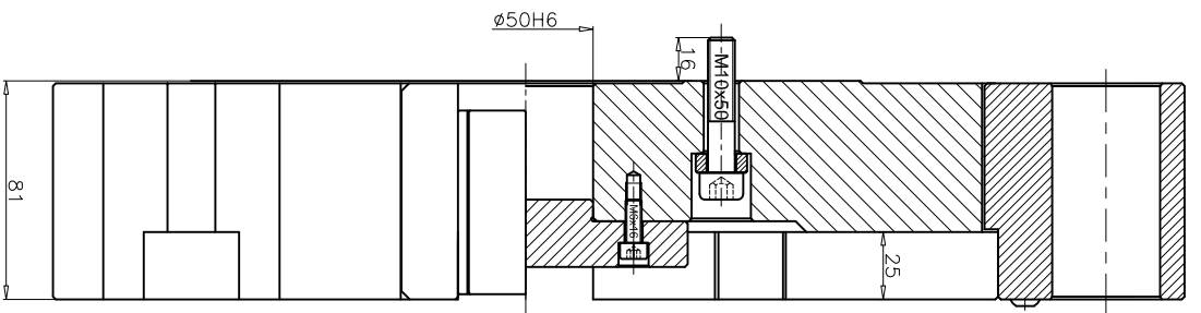
SECTION - FF
